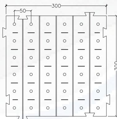
Hazard Drilling Template
