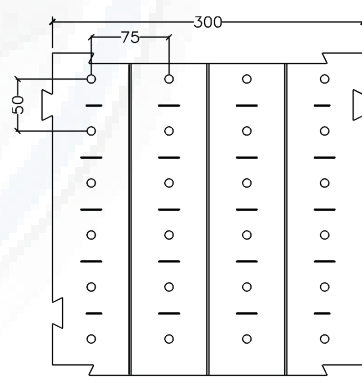
Directional Drilling Template
